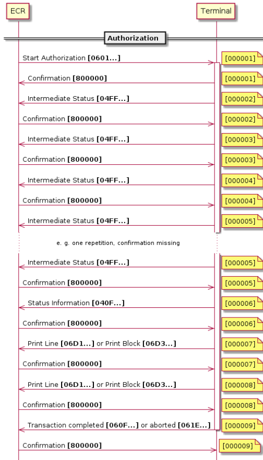
Message flow between ecr and terminal ZVT cash register protocol with message sequence id
